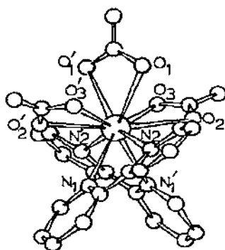
Fig. 1. Molecular structure of \text{La}(\text{bipy})_2(\text{NO}_3)_3 . Reprinted with permission of the authors and The American Chemical Society from A.R. Al-Karaghauli and J.S. Wood, J. Amer. Chem. Soc. , 90 (1968) 6548.
