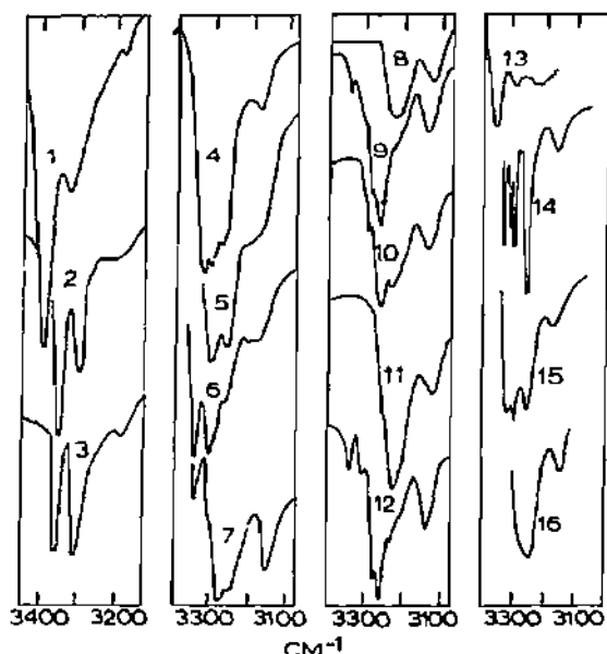
Fig. 5. Infrared spectra of \text{Ln}(\text{en})_n\text{X}_3 and \text{Ln}(\text{tren})_n\text{X}_3 species in the NH stretching region: 1, free en (soln.); 2, \text{Nd}(\text{en})_4(\text{ClO}_4)_3 ; 3, \text{Nd}(\text{en})_4(\text{ClO}_4)_3 (soln.); 4, [\text{Ln}(\text{en})_4\text{NO}_3](\text{NO}_3)_2 ; 5, [\text{Ln}(\text{en})_4](\text{NO}_3)_3 ; 6, [\text{Ln}(\text{en})_3(\text{NO}_3)_2]\text{NO}_3 ; 7, [\text{Ln}(\text{en})_4\text{Cl}]\text{Cl}_2 ; 8, [\text{Ln}(\text{en})_4]\text{Cl}_3 ; 9, [\text{Ln}(\text{en})_3\text{Cl}_2]\text{Cl} ; 10, [\text{La}(\text{en})_4\text{Br}]\text{Br}_2 ; 11, [\text{Ln}(\text{en})_4]\text{Br}_3 ; 12, [\text{Ln}(\text{en})_3\text{Br}_2]\text{Br} ; 13, free tren; 14, [\text{Ln}(\text{tren})(\text{NO}_3)_3] ; 15, [\text{Ln}(\text{tren})_2\text{NO}_3](\text{NO}_3)_2 ; 16, [\text{Ln}(\text{tren})_2](\text{NO}_3)_3 . Reprinted with permission of The American Chemical Society from J.H. Forsberg and T. Moeller, Inorg. Chem. , 8 (1969) 883 and J.H. Forsberg, T.M. Kubik, T. Moeller and K. Gucwa, Inorg. Chem. , 10 (1971) 2656.
